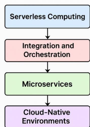
Fig. 1. Proposed Methodology
